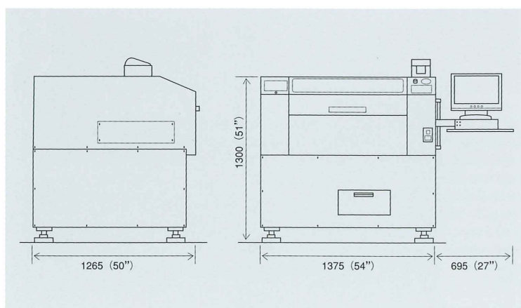
APT-9411CE-A WITH SHUTTLE CONVEYER STATION
